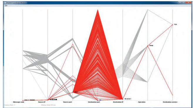
Figure 5: IRC traffic at source port 6667. This is the snap shot of Parallel Coordinated Window at 4/6/2012 15:00:06 during 1000 second period. The highlight filter is "Source port = 6667". These accesses use the random destination ports.
